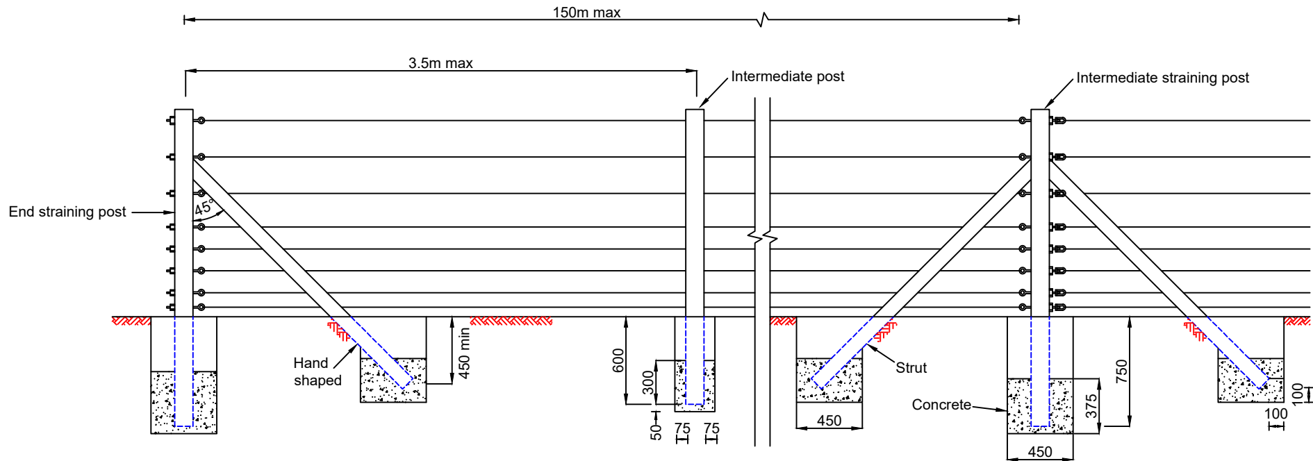
TYPICAL CONSTRUCTION DETAILS (TYPE ILLUSTRATED REF SC 135B - CONCRETE POSTS)
