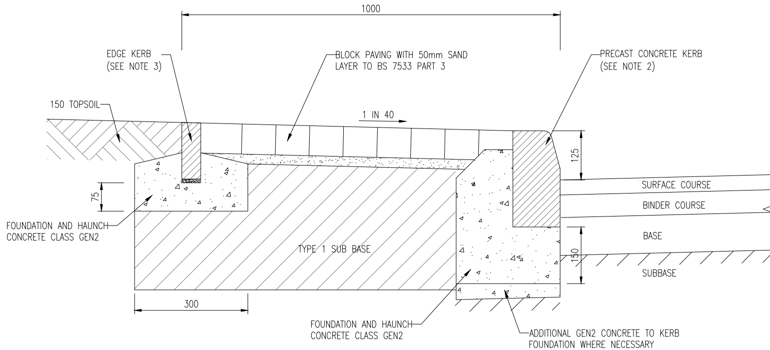
HARD VERGE DETAIL (SCALE 1:10)
