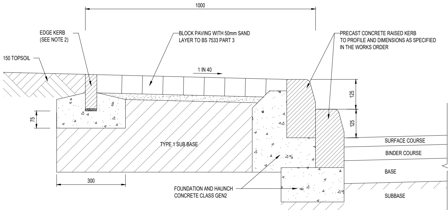
RAISED KERB HARD EDGE DETAIL (SCALE 1:10)
