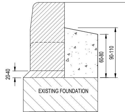
DL1/DR1 PRECAST CONCRETE KERB TO BE EN 1340 TYPE R1 (DROPPER KERB) (SCALE 1:10)
