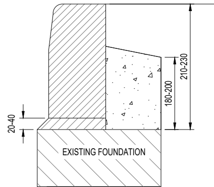
HB2 PRECAST CONCRETE KERB TO BS EN 1340 TYPE RG. (SCALE 1:10)
