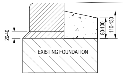
BN PRECAST CONCRETE KERB TO BE EN 1340 TYPE RH. (SCALE 1:10)
