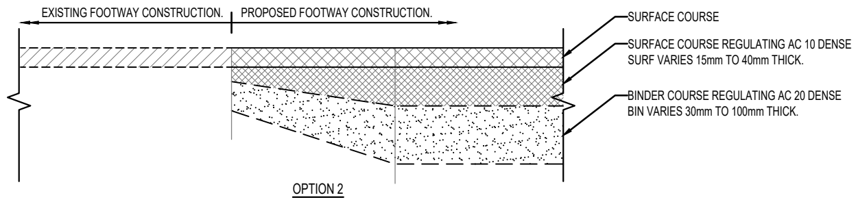
FOOTWAY TYPE 3 (SCALE 1:10)
