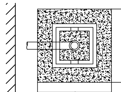
PLAN DETAIL OF LOOP DETECTOR BOX
