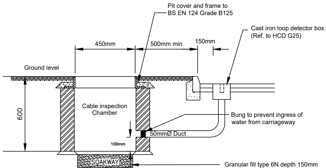
DETAIL OF LOOP CABLE PIT AND DUCT
