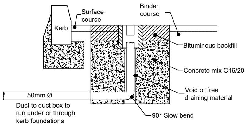
TYPICAL CROSS SECTION DETAIL THROUGH LOOP DETECTOR BOX
