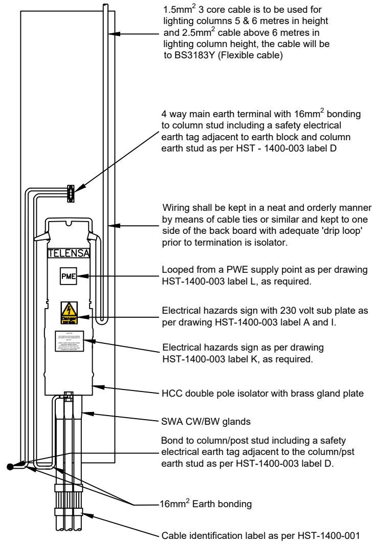
HCC SERVICE SINGLE ARM COLUMN WITH SUBFUSE
