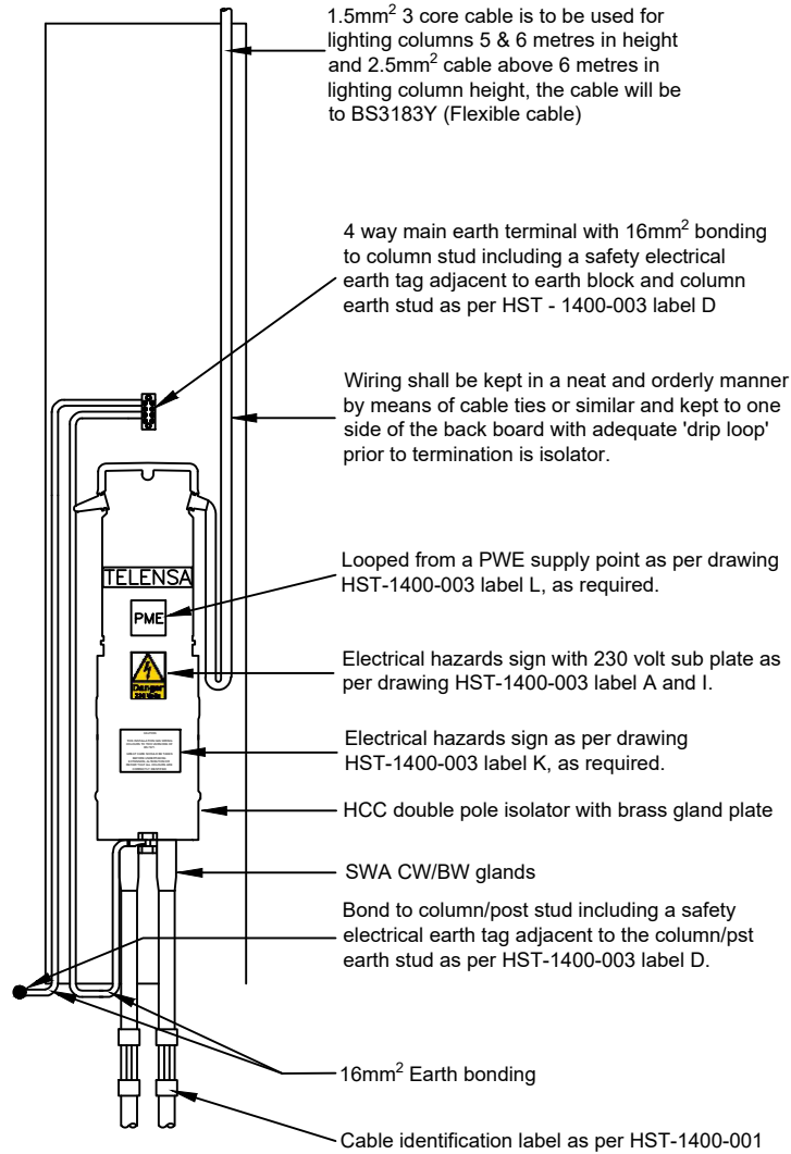
HCC SERVICE SINGLE ARM COLUMN
