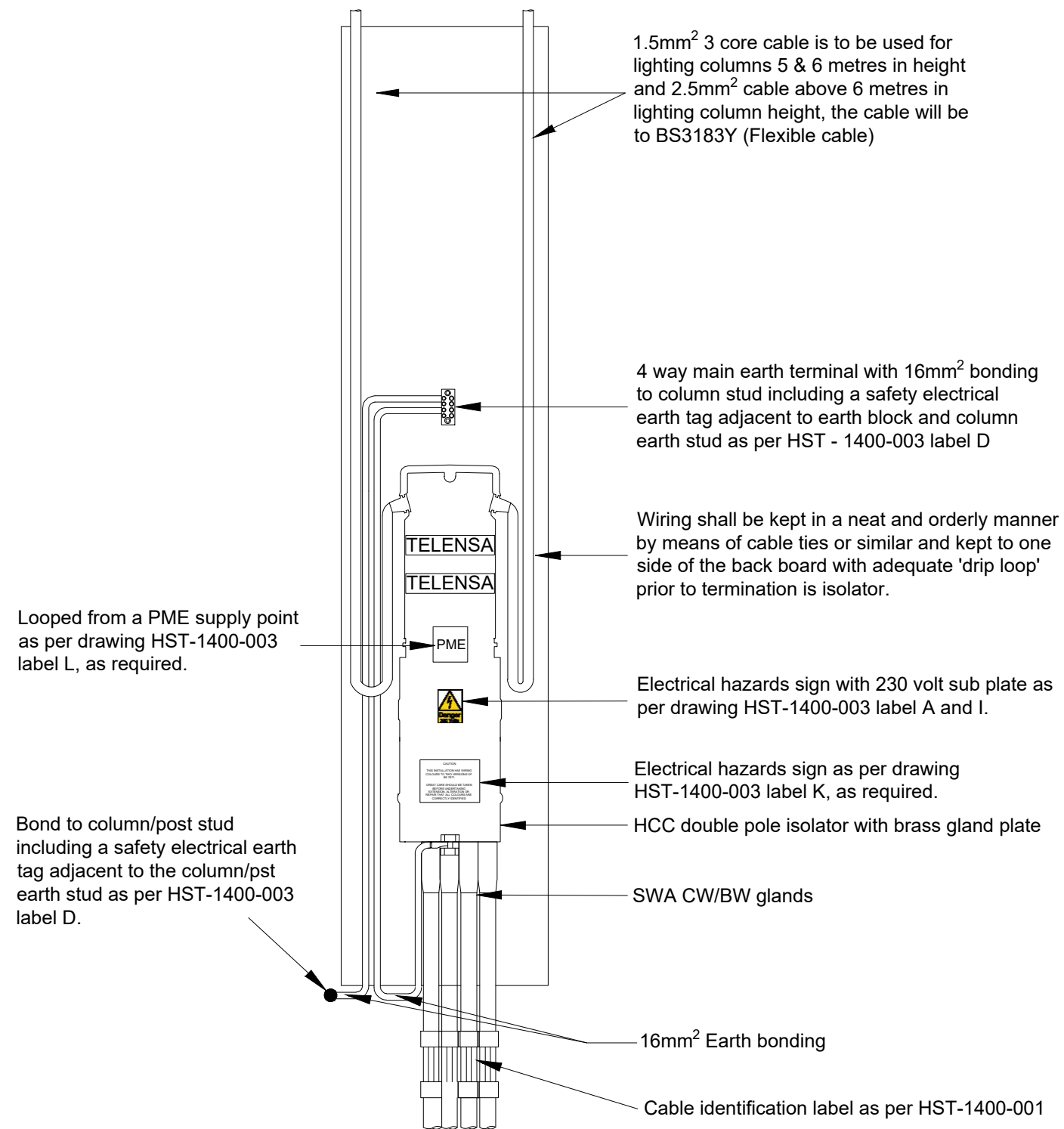
HCC SERVICE DOUBLE ARM COLUMN WITH TWO SUBFUSES
