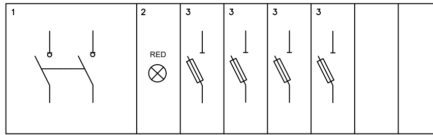
GROUP SWITCHING PANEL
