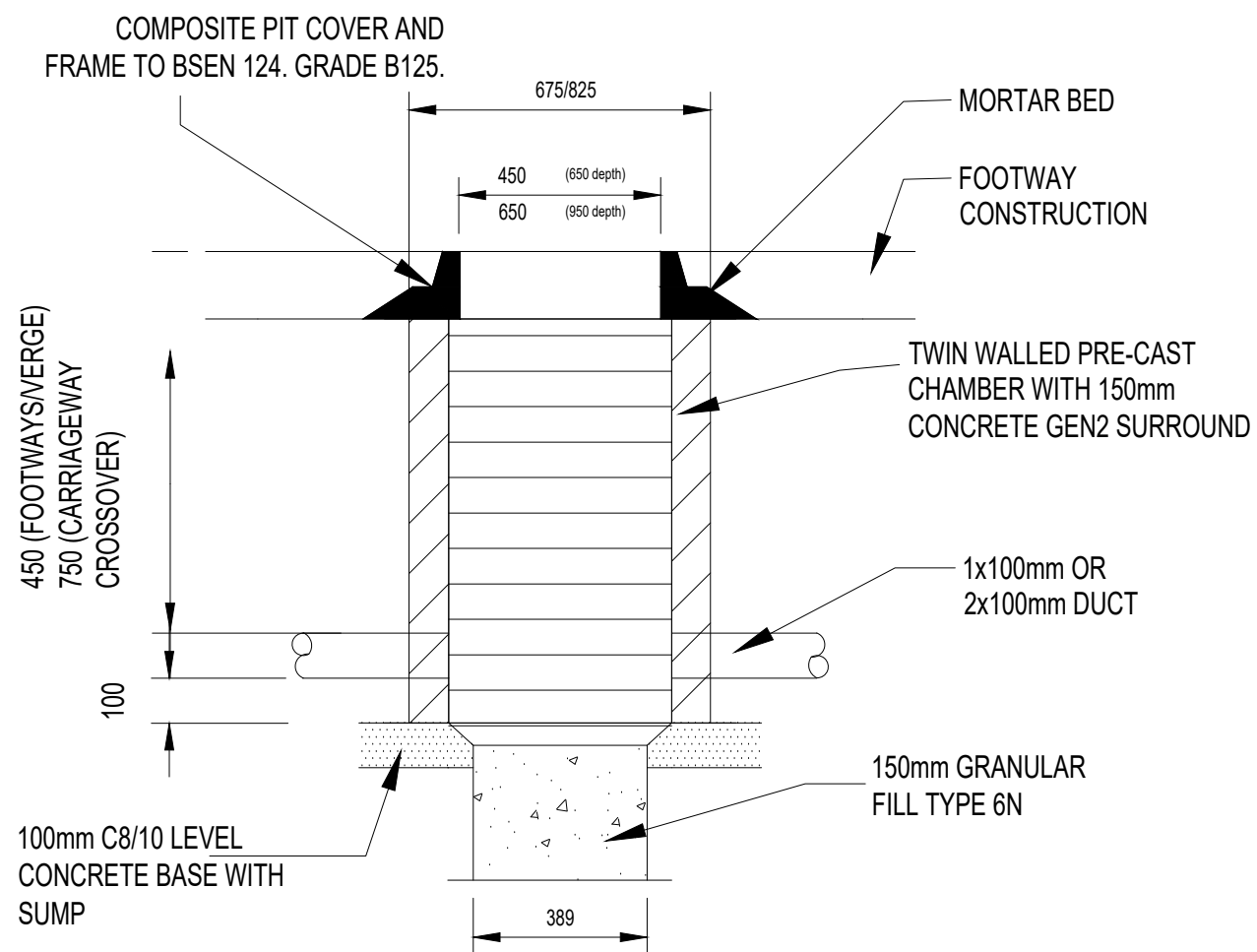
DETAIL OF CABLE PIT AND DUCT
